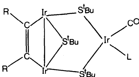
Fig. 2. The complexes studied by Lemoine et al. [42]: \text{L}=\text{CO} , \text{R}=\text{CF}_3 complex I; \text{L}=\text{CO} , \text{R}=\text{COOMe} complex II; \text{R}=\text{CF}_3 , \text{L}=\text{C}_4\text{F}_6 complex III; \text{R}=\text{CF}_3 , \text{L}=\text{POMe}_3 complex IV.
