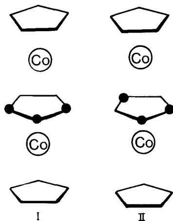
Fig. 6. The complexes studied by Brennan and Geiger [59]. (●=BH); I=1, 7, 2, 3- (\eta^5\text{-C}_5\text{H}_5)\text{Co}_2\text{C}_2\text{B}_3\text{H}_5 ; II=1, 7, 2, 4- (\eta^5\text{-C}_5\text{H}_5)\text{Co}_2\text{C}_2\text{B}_3\text{H}_5 .
