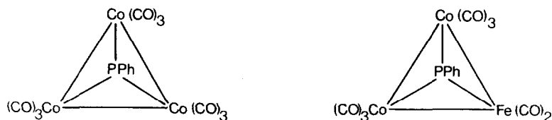
Fig. 5. Triangular clusters studied by Vahrenkamp and co-workers [58].
